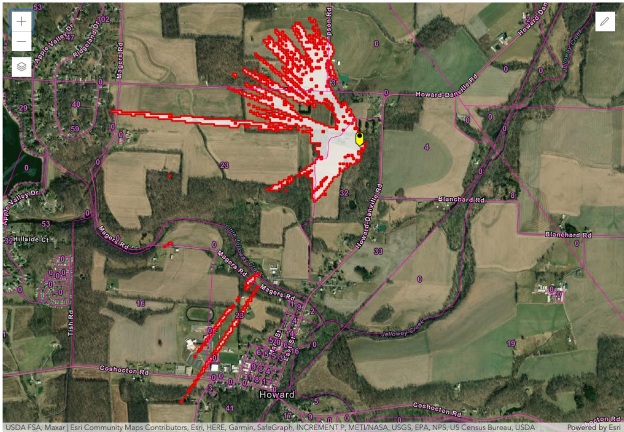
Figure 1 – Howard, OH SAN -77.6 dB(mW/(m 2 * MHz)) pfd contour
