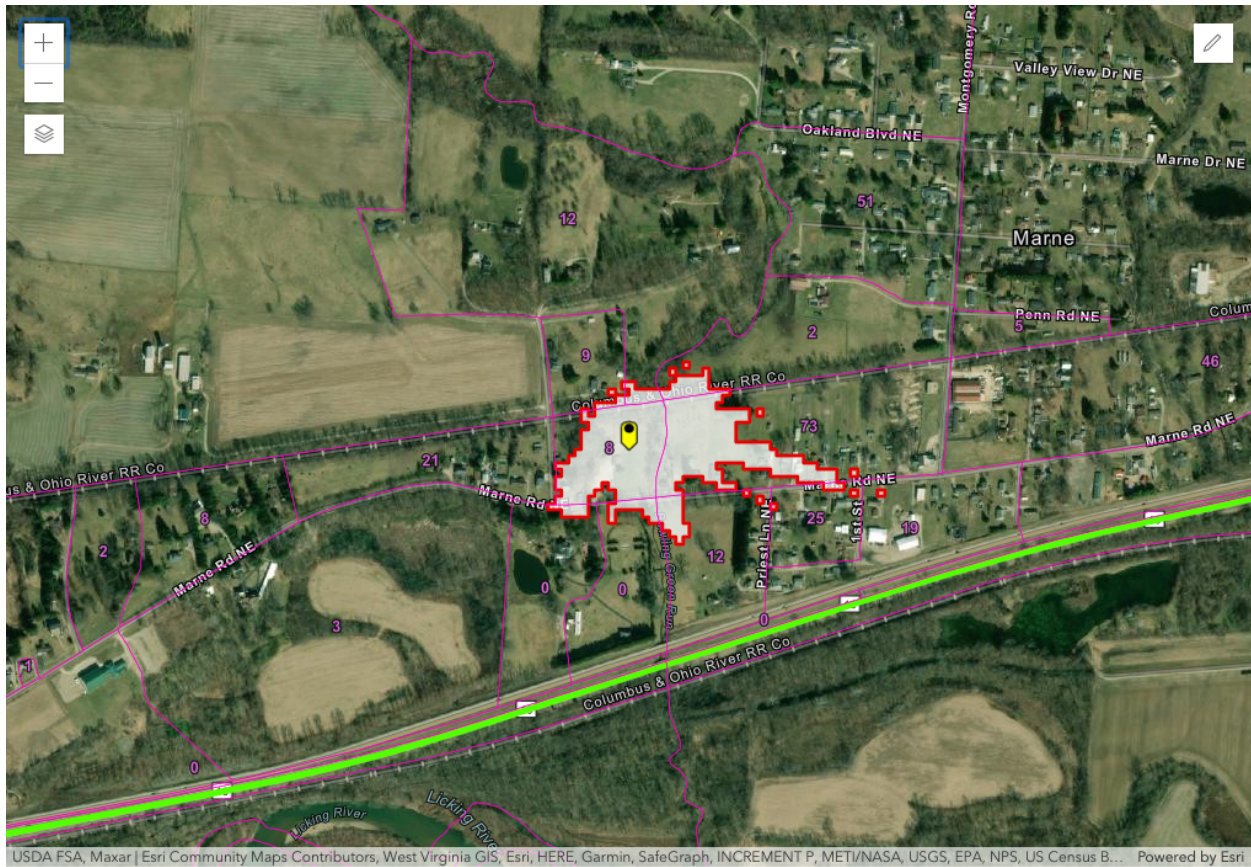
Figure 1 – Newark, OH SAN -77.6 dB(mW/(m 2 * MHz)) pfd contour
