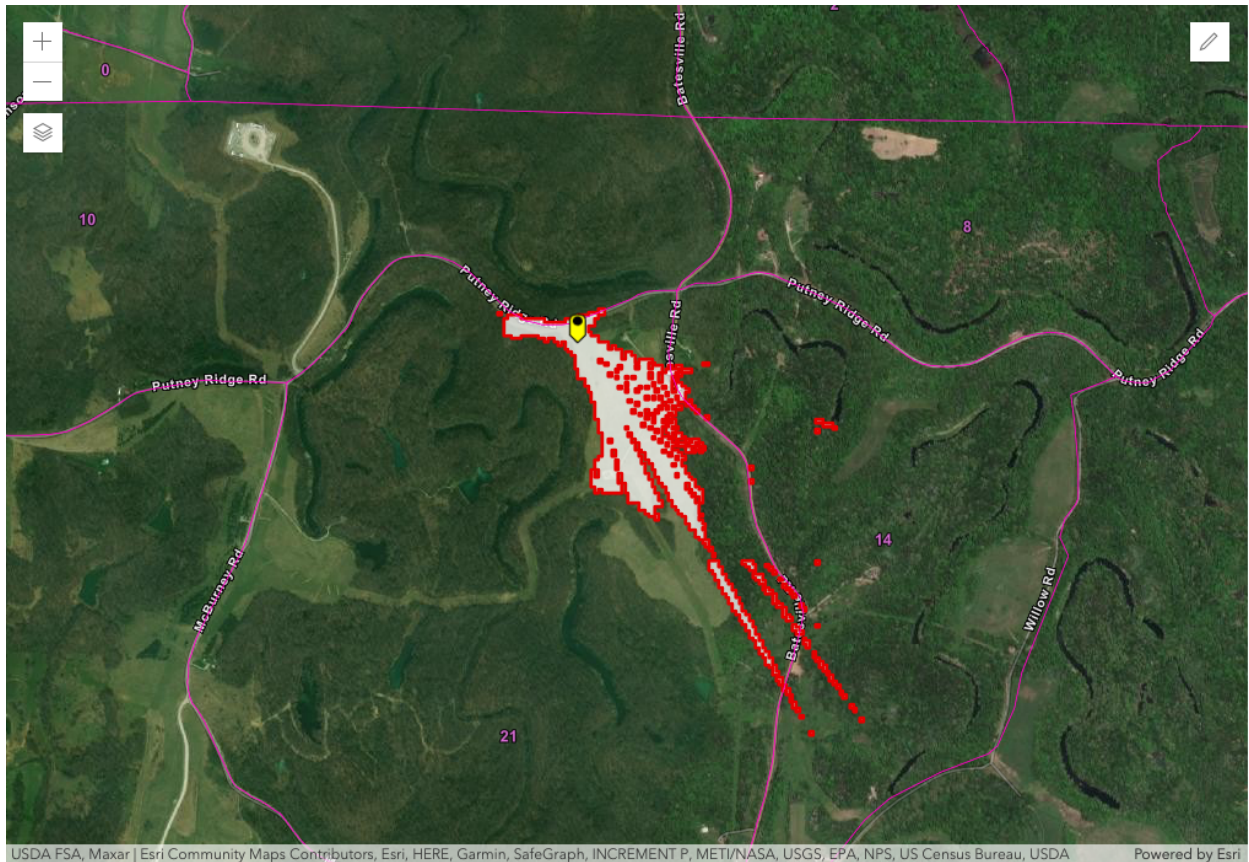
Figure 1 – Quaker City, OH SAN -77.6 dB(mW/(m 2 * MHz)) pfd contour
