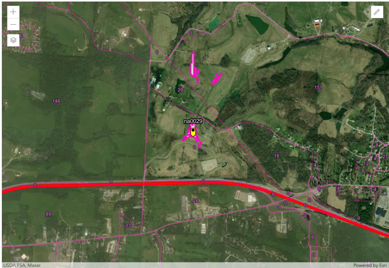
Figure 1 – Saint Clairsville, OH SAN -77.6 dB(mW/(m 2 * MHz)) pfd contour
