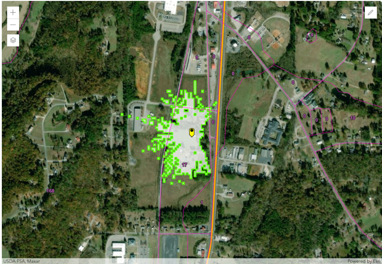
Figure 1 – Rock Spring, GA SAN -77.6 dB(mW/(m 2 * MHz)) pfd contour
