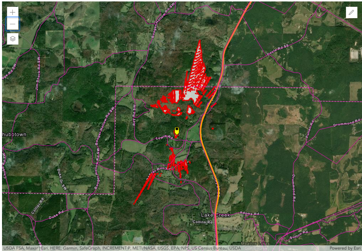
Figure 1 – Cedartown, GA SAN -77.6 dB(mW/(m 2 * MHz)) pfd contour
