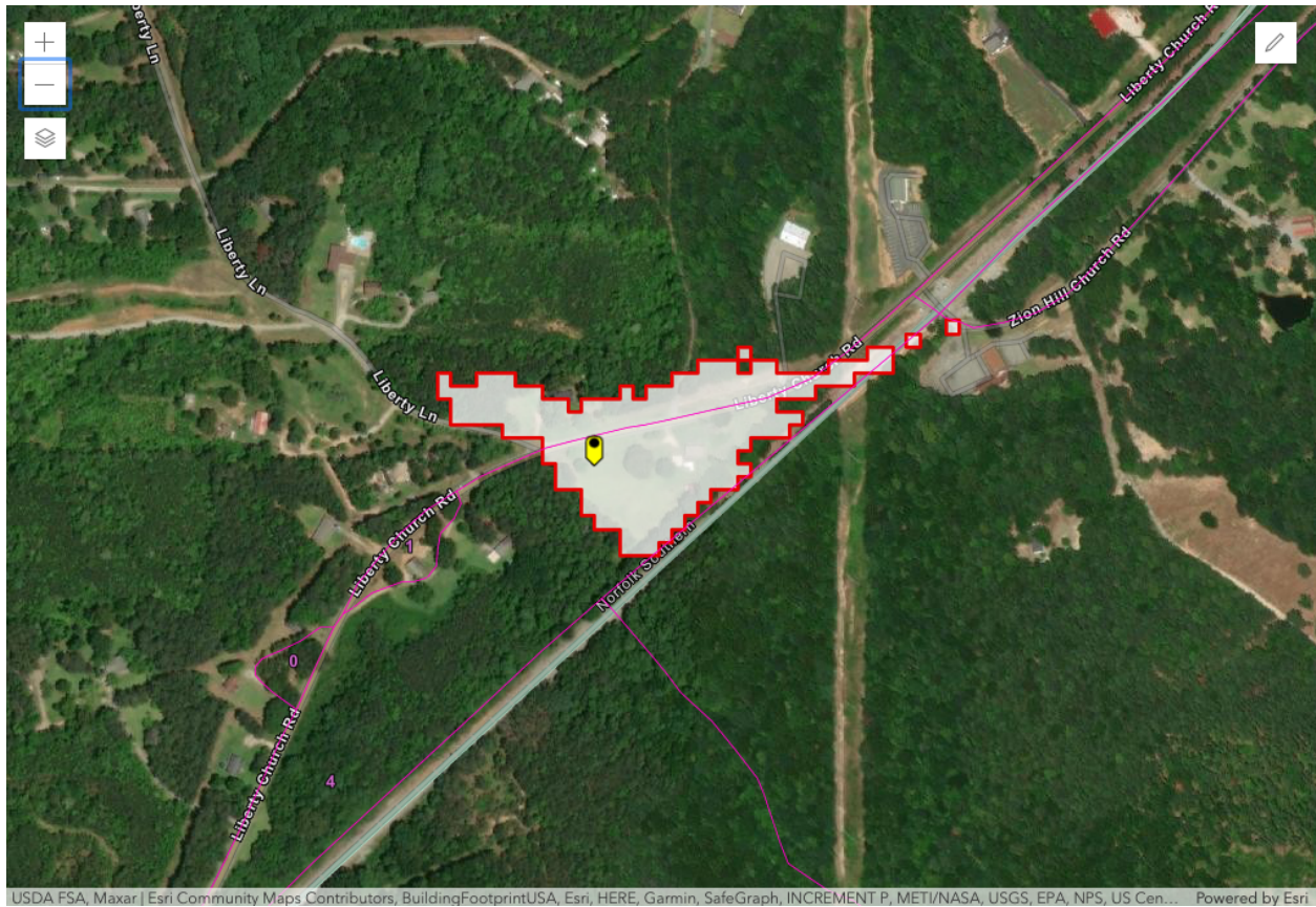
Figure 1 – Bremen, GA SAN -77.6 dB(mW/(m 2 * MHz)) pfd contour
