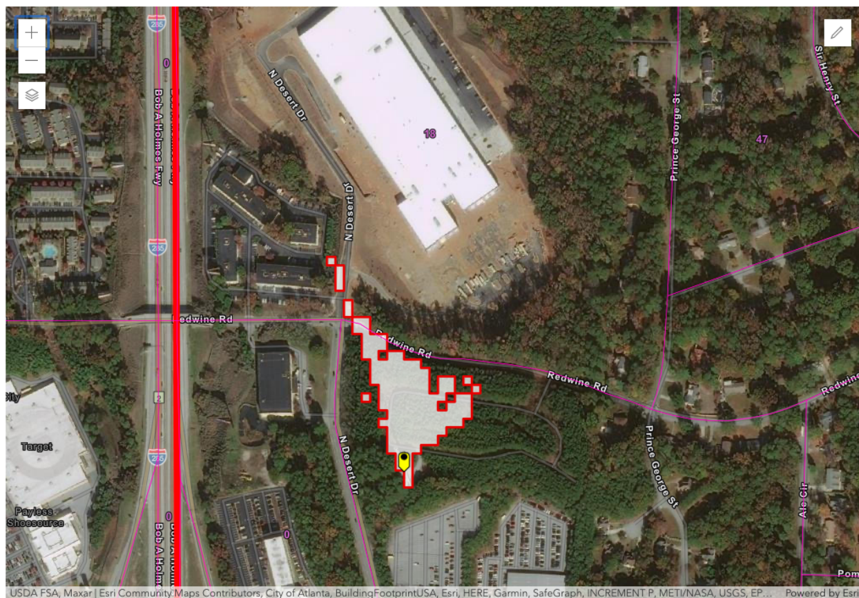
Figure 1 – East Point, GA SAN -77.6 dB(mW/(m 2 * MHz)) pfd contour
