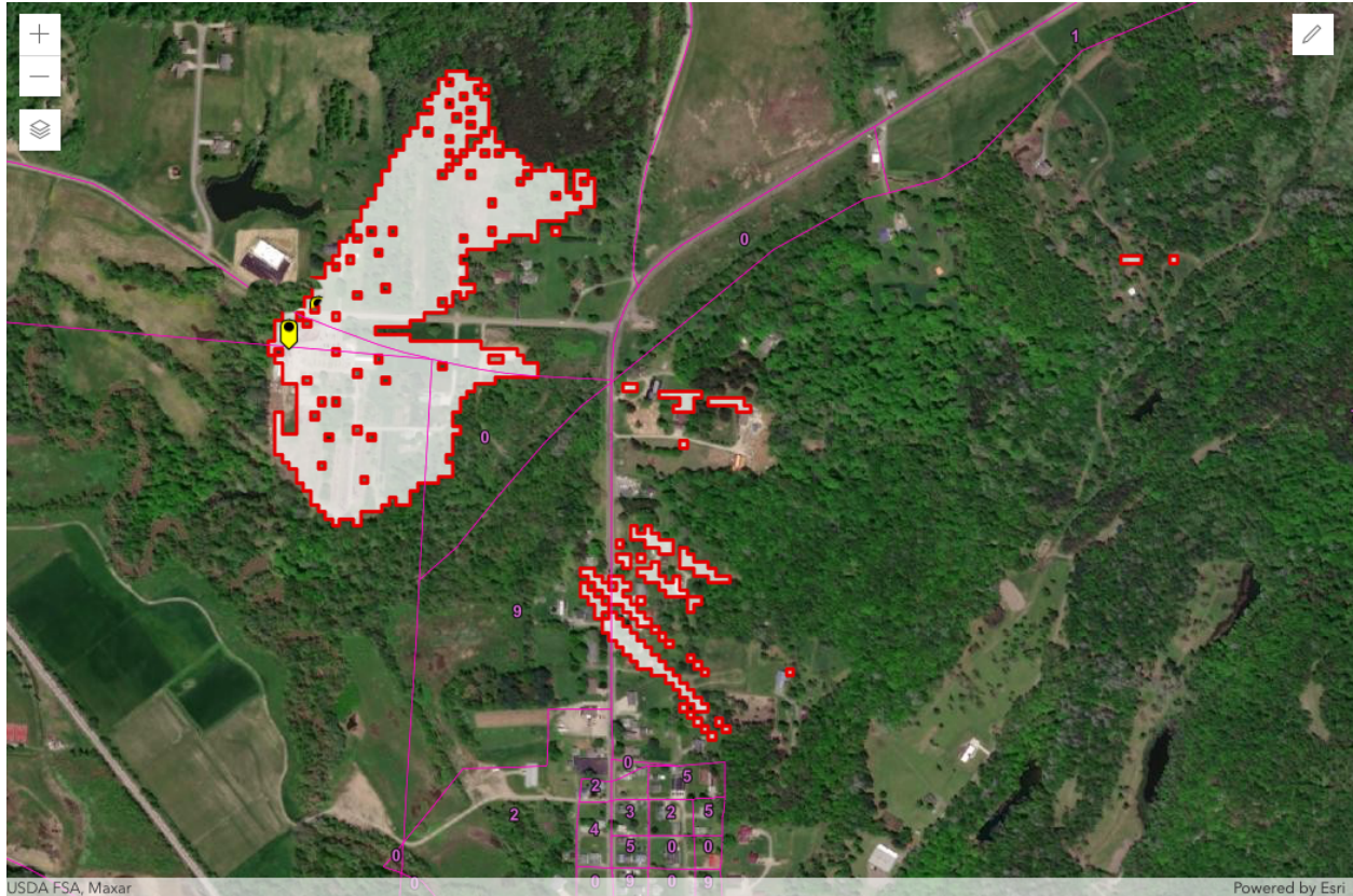
Figure 1 – Sherrodsville, OH SAN -77.6 dB(mW/(m 2 * MHz)) pfd contour
