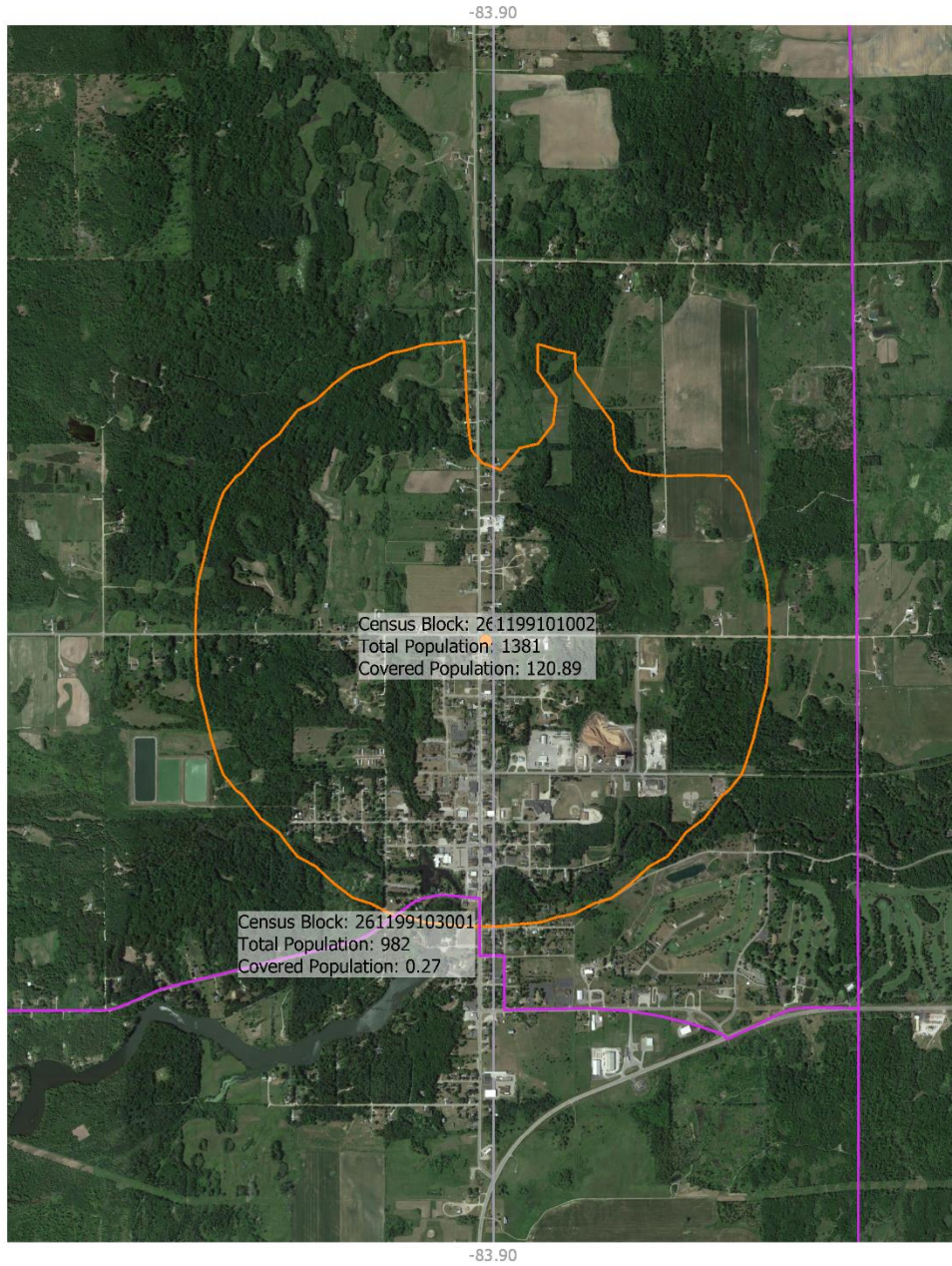
Figure 1. PFD Contours for Hillman Gateway
