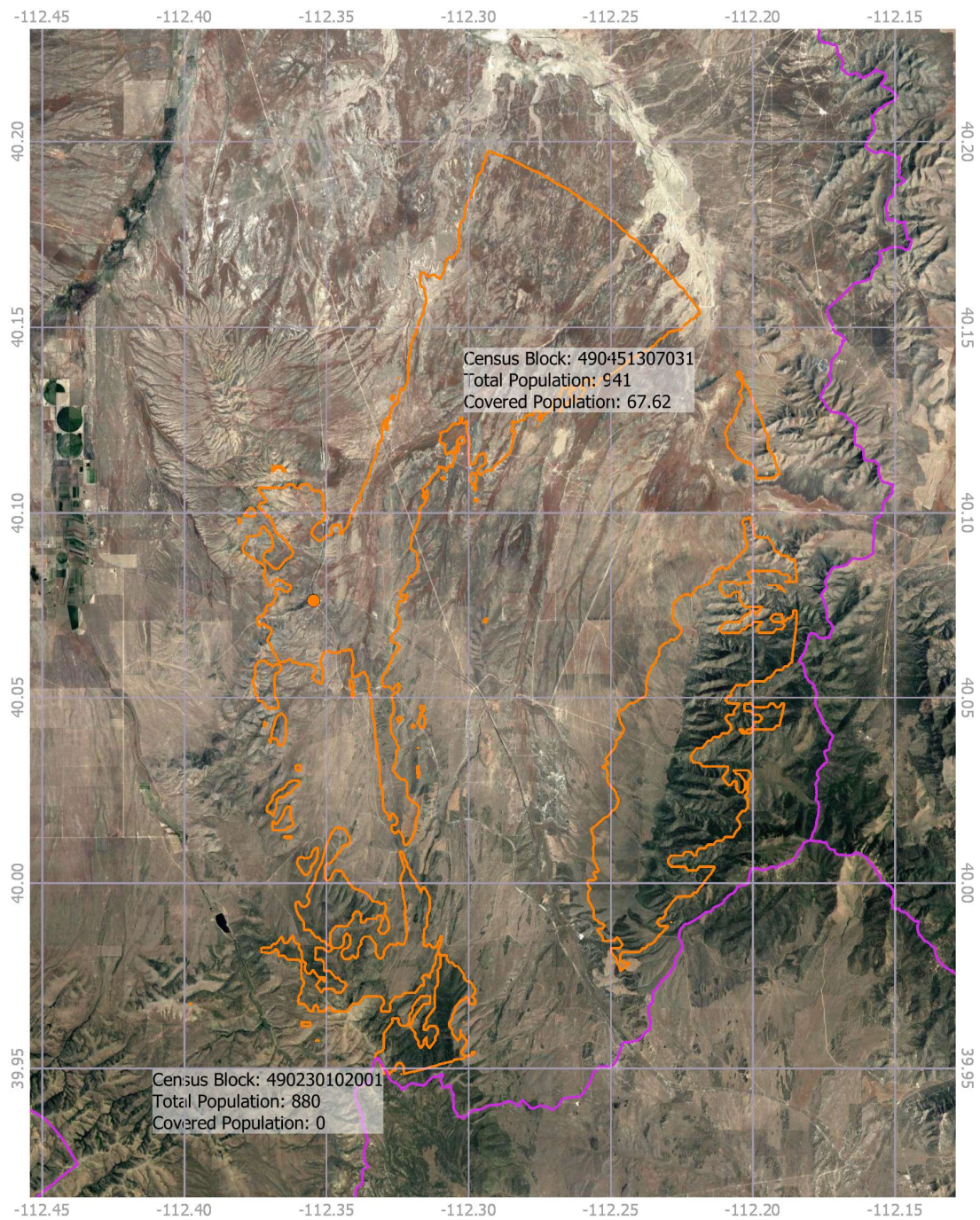
Figure 1. PFD Contours for Vernon Gateway
