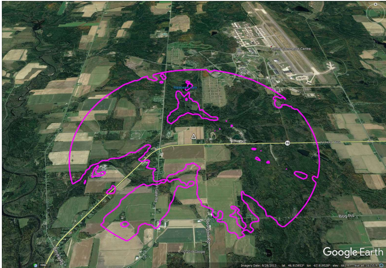
Figure 1. PFD Contours for Loring Gateway
