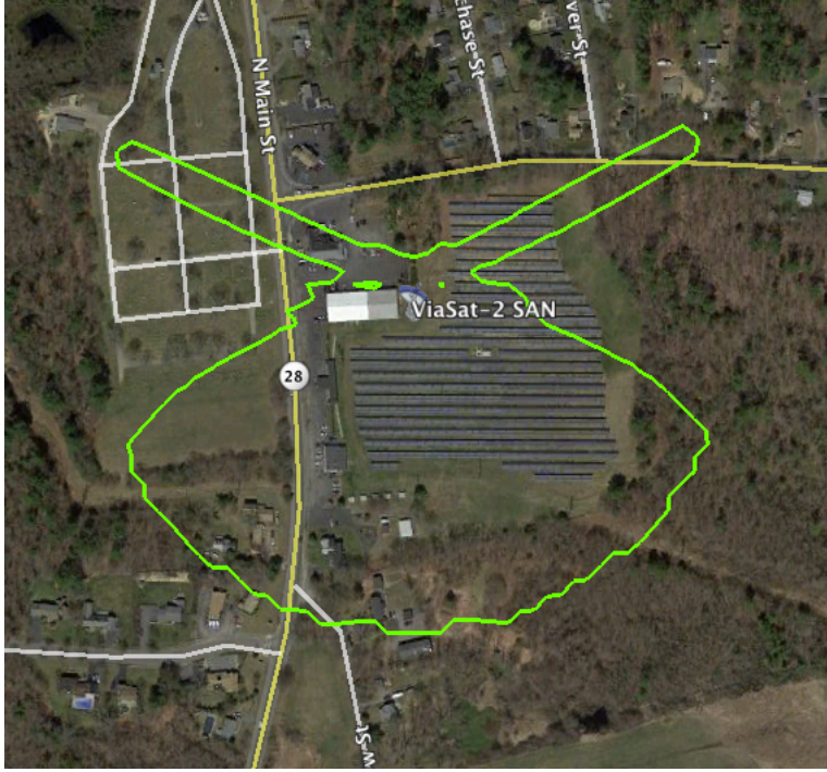
Figure 2 – West Bridgewater SAN -77.6 dBm/(m 2 * MHz) PFD contour
