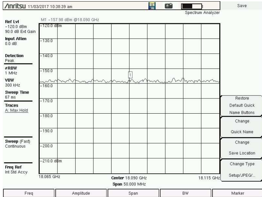
Spectrum Photos 18.090 GHz 1 MHz Res BW Vertical Pol AZ 92.6 0
