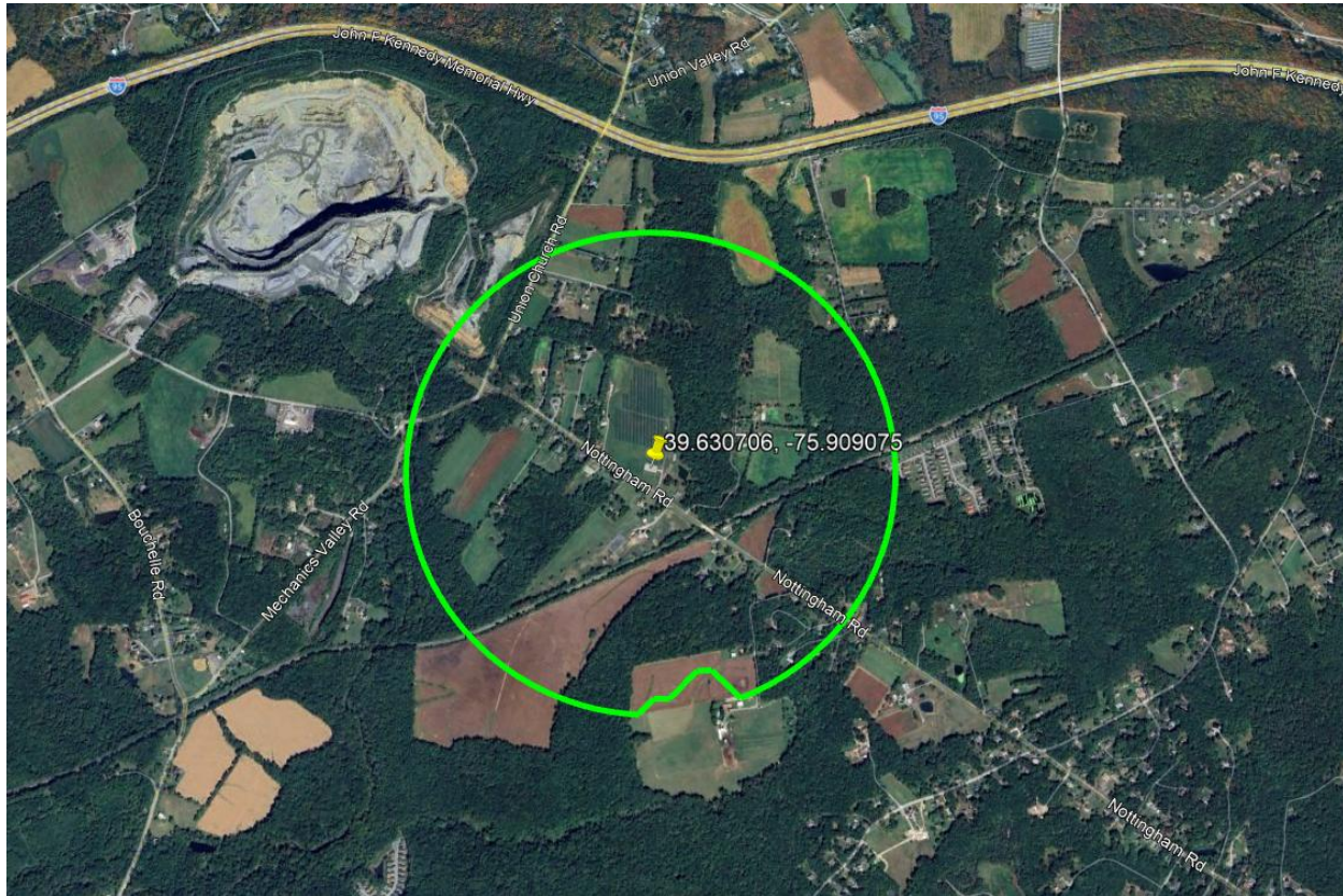
Figure 1. PFD Contour for the Gateway: V-band (47.2 GHz)
