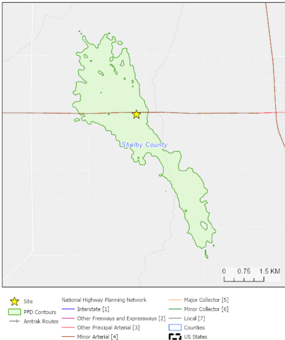
Figure 4. -77.6 dBm/m 2 /MHz PFD contour overlaid with major roadways and passenger railroads 24
