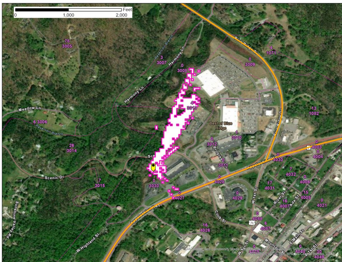
Figure 1 – Blue Ridge, GA SAN -77.6 dB(mW/(m 2 * MHz)) pfd contour
