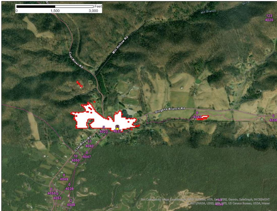
Figure 1 – Glen Daniel, WV SAN -77.6 \text{ dB(mW/(m}^2 * \text{MHz))} pfd contour
