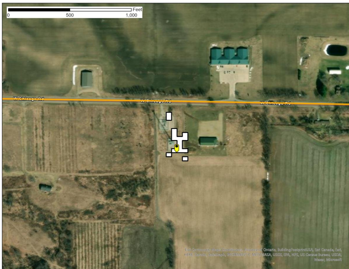
Figure 1 – Allen, MI SAN -77.6 dB(mW/(m² * MHz)) pfd contour
