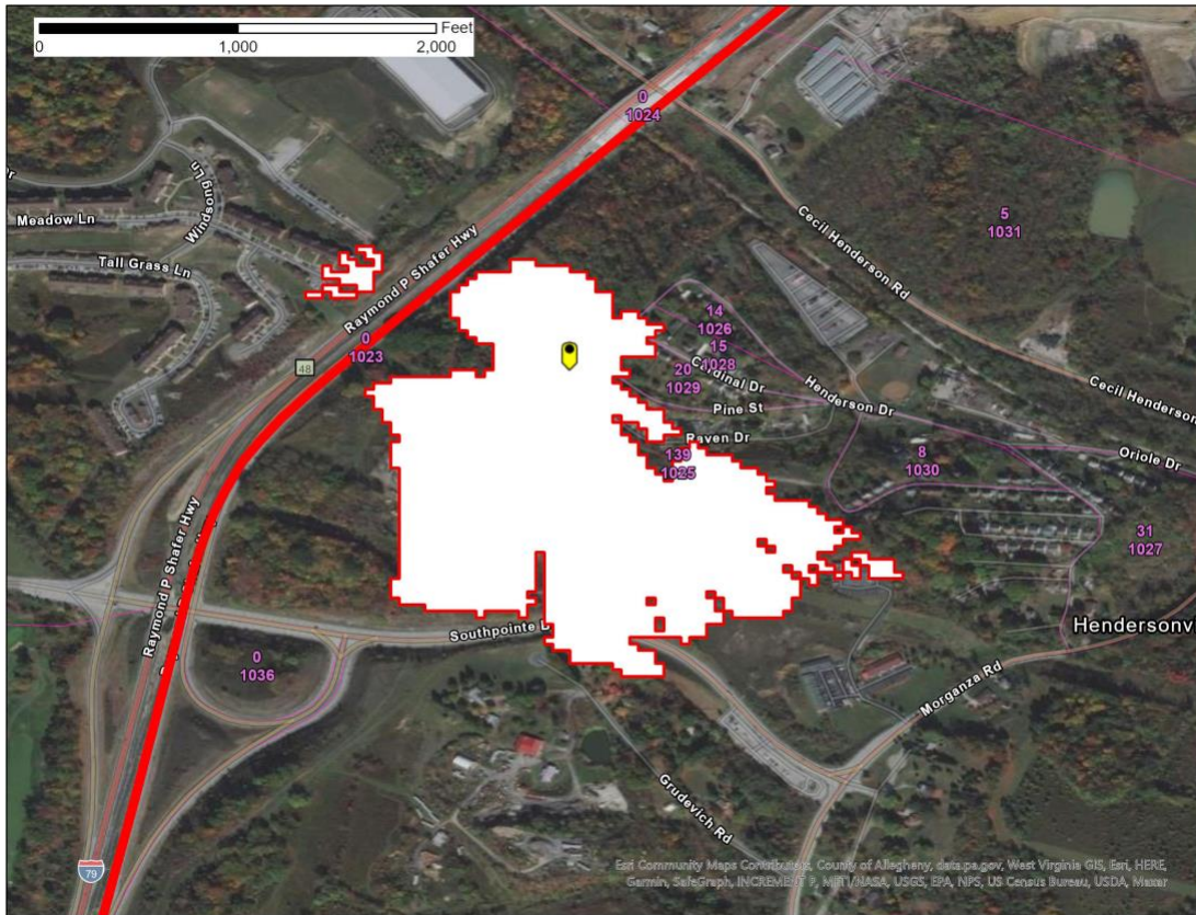
Figure 1 – Canonsburg, PA SAN -77.6 \text{ dB(mW/(m}^2 * \text{MHz))} pfd contour
