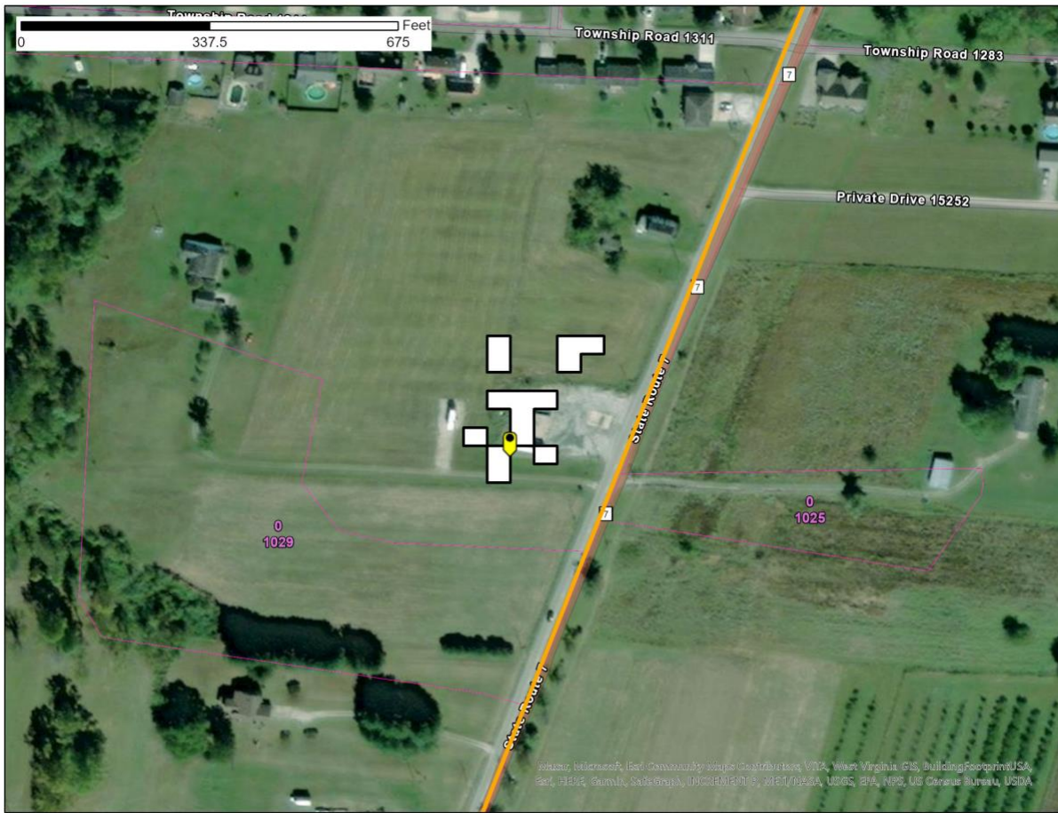
Figure 1 – Proctorville, OH SAN -77.6 dB(mW/(m² * MHz)) pfd contour
