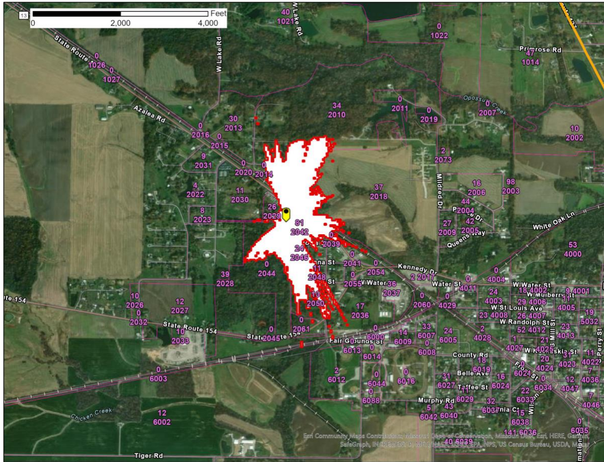
Figure 1 – Pinckneyville, IL SAN -77.6 dB(mW/(m 2 * MHz)) pfd contour
