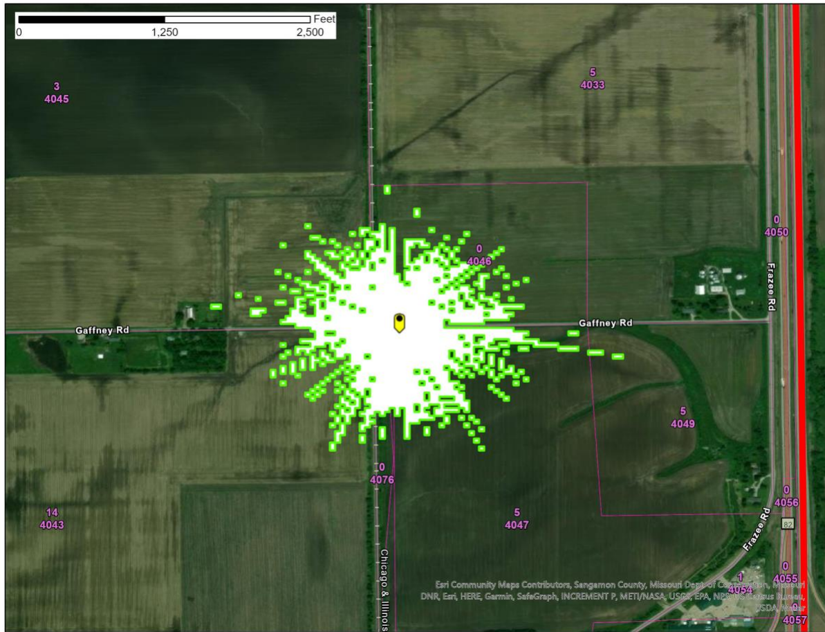
Figure 1 – Divernon, IL SAN -77.6 dB(mW/(m 2 * MHz)) pfd contour
