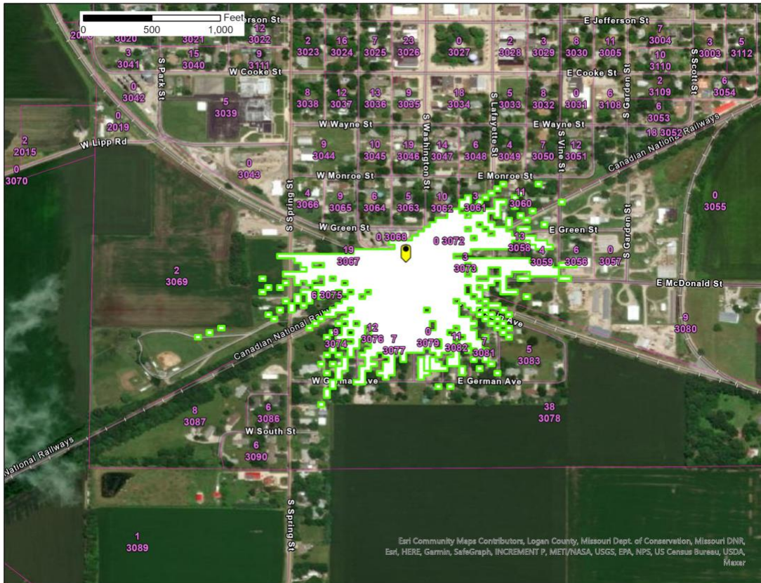
Figure 1 – Mt Pulaski, IL SAN -77.6 \text{ dB(mW/(m}^2 * \text{MHz))} pfd contour
