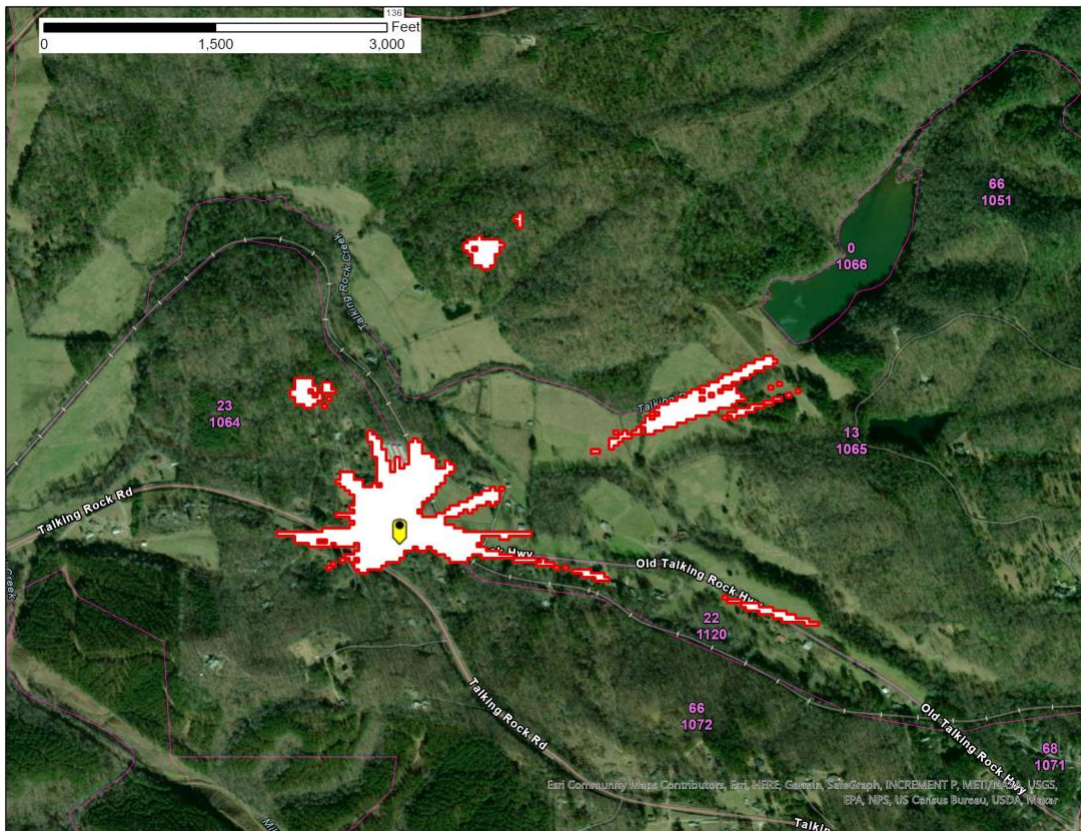
Figure 1 – Talking Rock, GA SAN -77.6 \text{ dB(mW/(m}^2 * \text{MHz))} pfd contour
