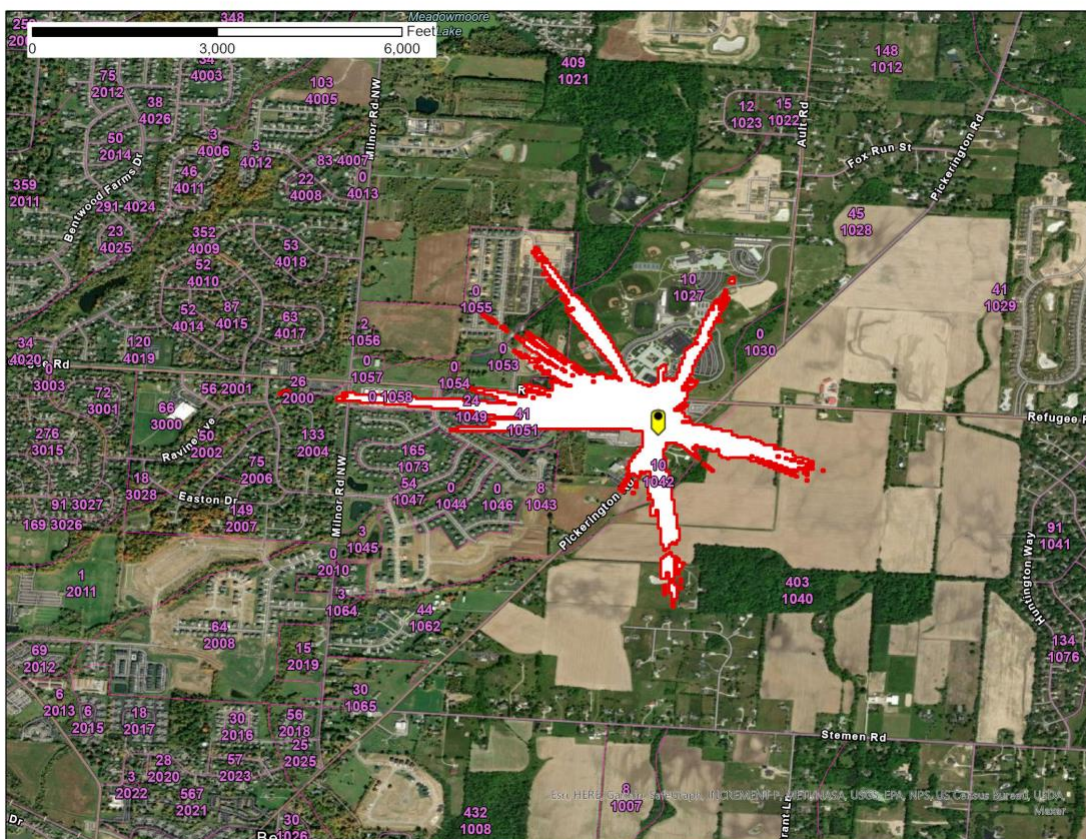
Figure 1 – Pickerington, OH SAN -77.6 \text{ dB(mW/(m}^2 * \text{MHz))} pfd contour
