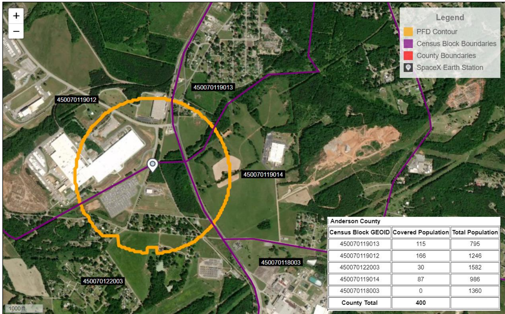
Figure 2. PFD Contour and Population Coverage
