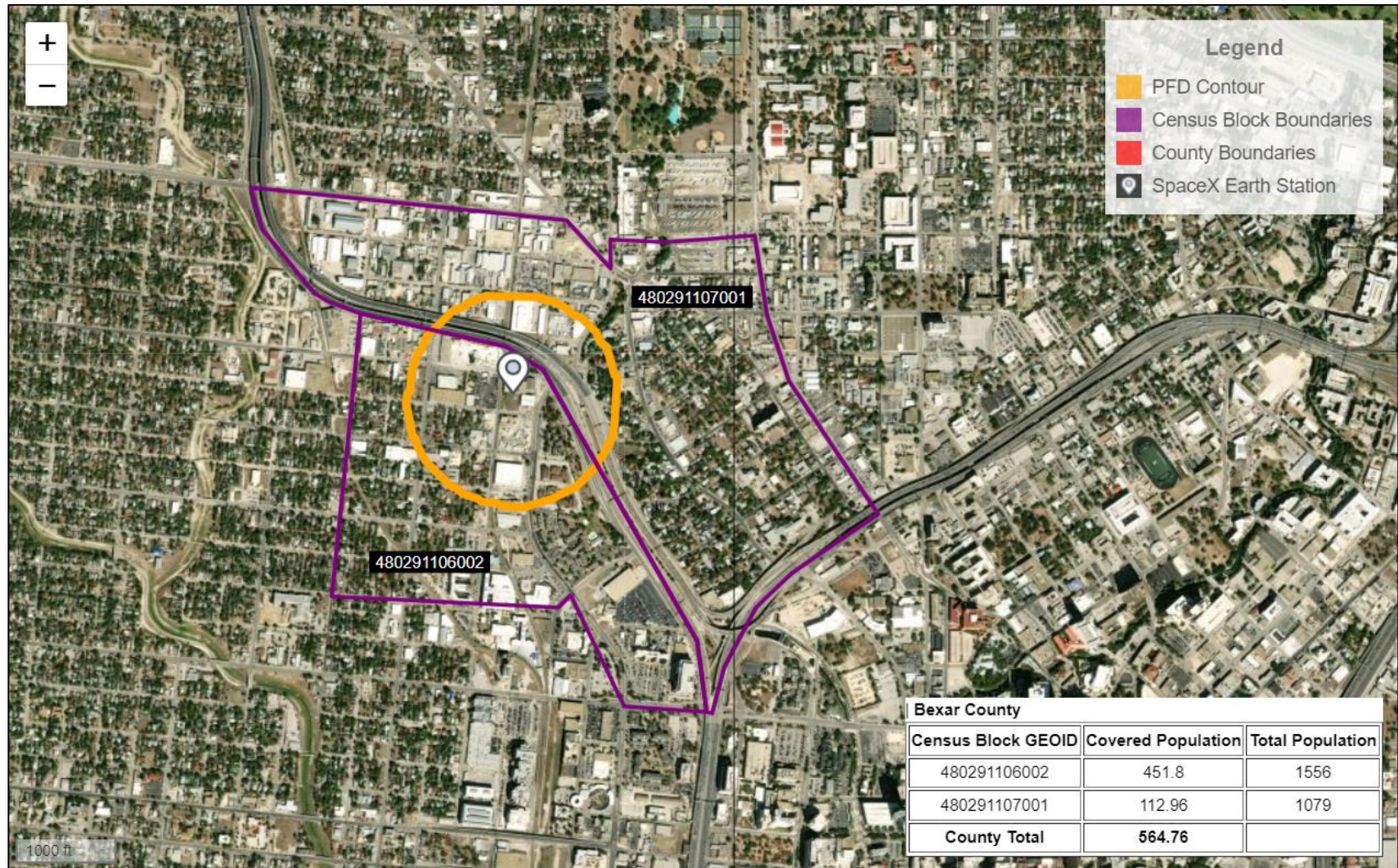
Figure 4. PFD Contour and Population Coverage for Grandfathered Gateway
