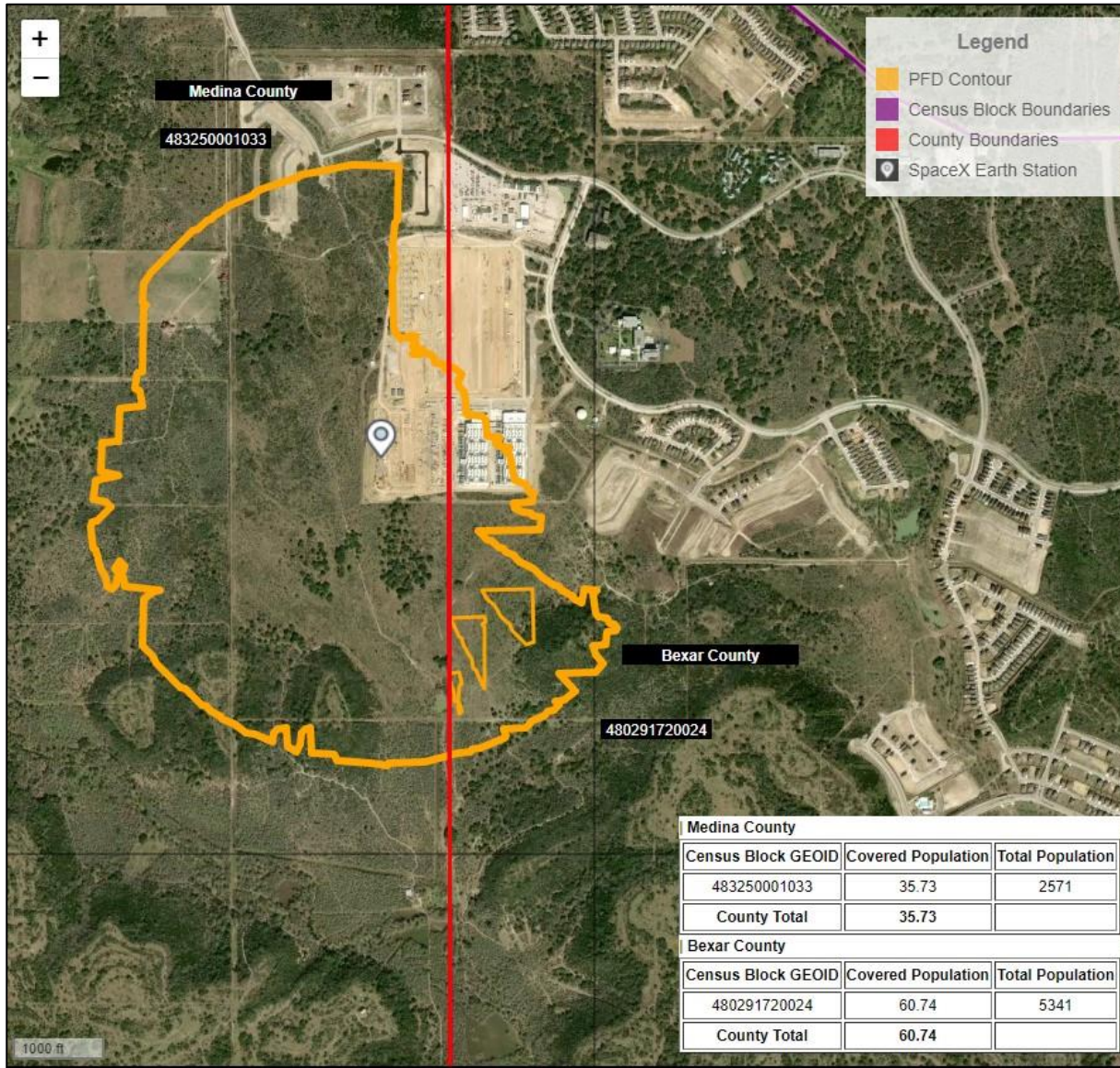
Figure 2. PFD Contour and Population Coverage for SpaceX Gateway
