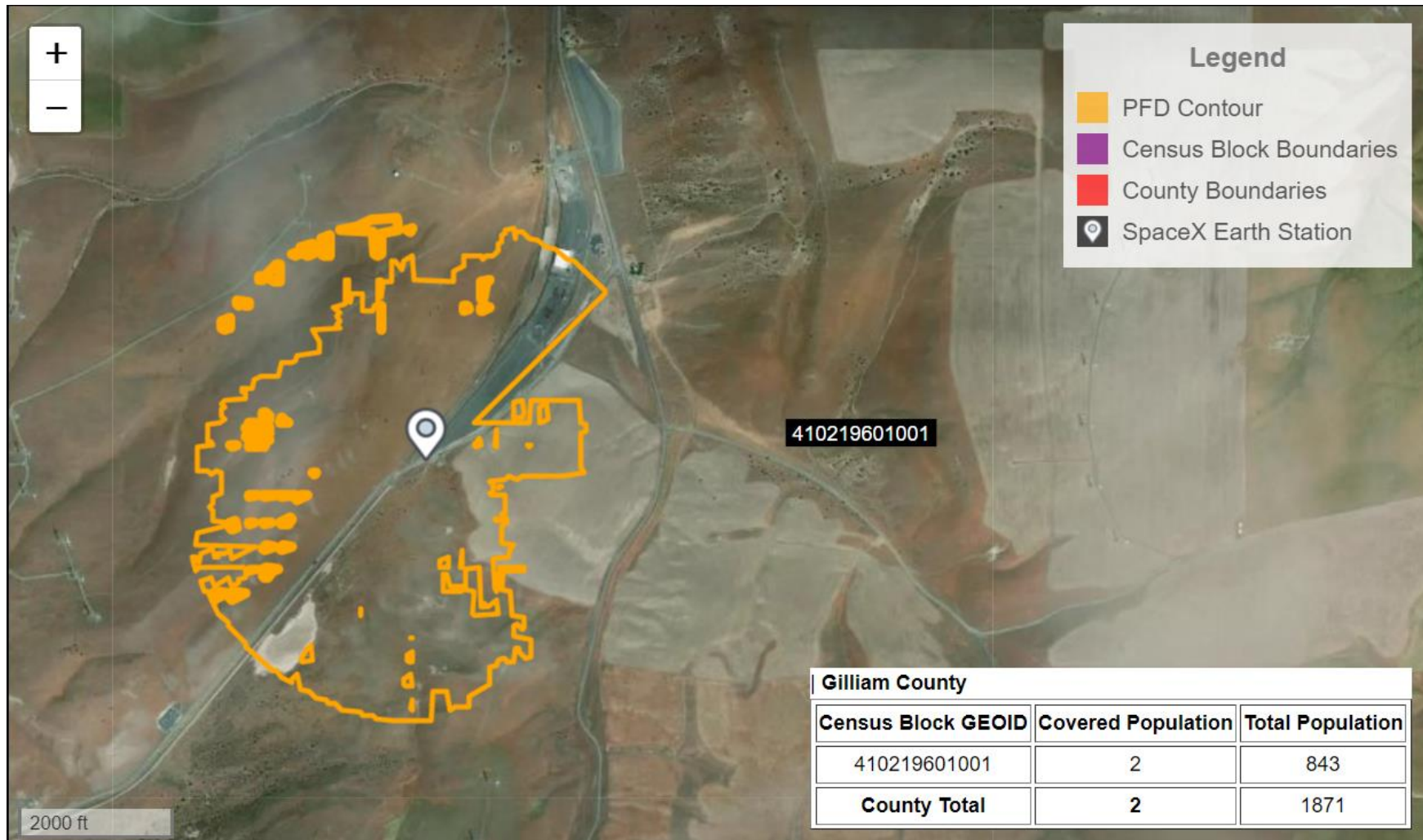
Figure 2. PFD Contour and Population Coverage
