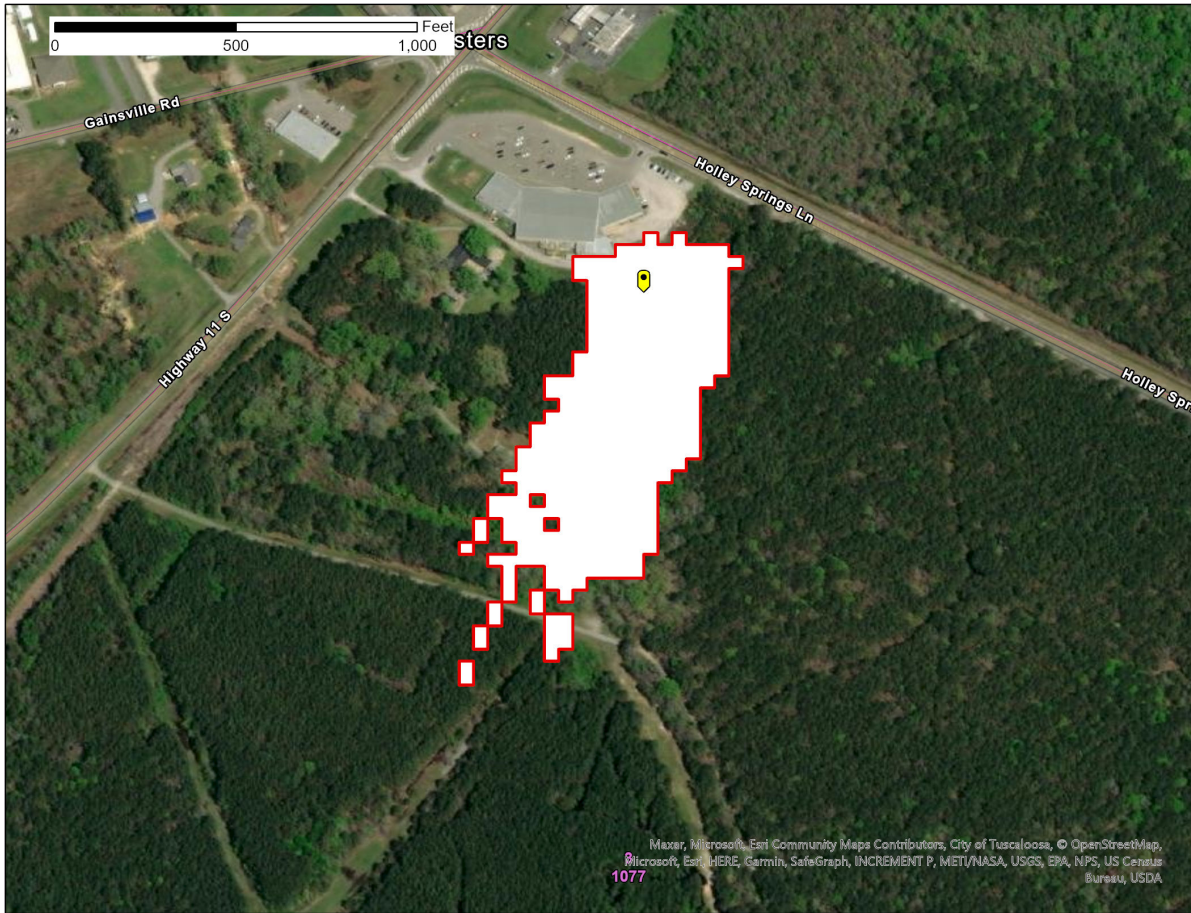
Figure 1 – Fosters, AL SAN -77.6 dB(mW/(m 2 * MHz)) pfd contour
