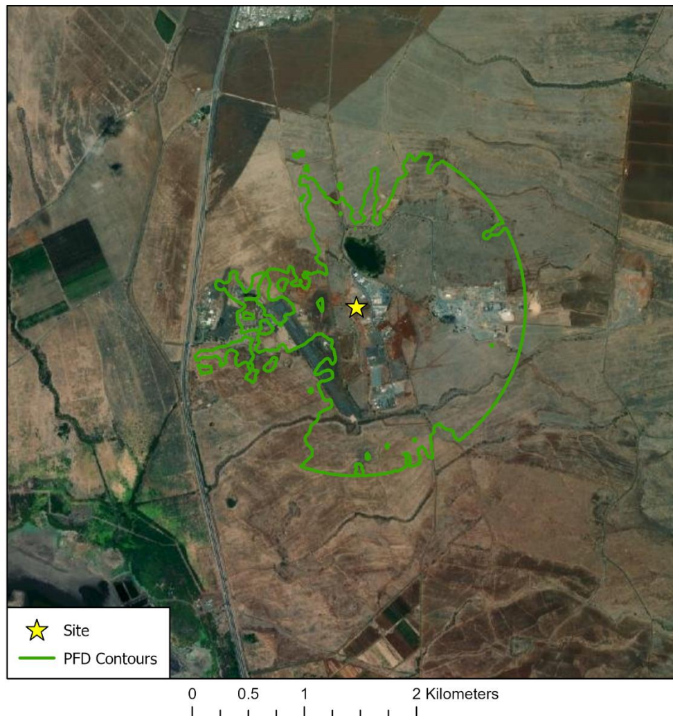
Figure 2. Gateway PFD Contour (-77.6 dBW/m 2 /MHz)
