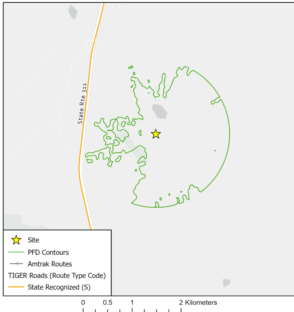
Figure 4. -77.6 dBm/m 2 /MHz PFD contour overlaid with major roadways and passenger railroads 28
