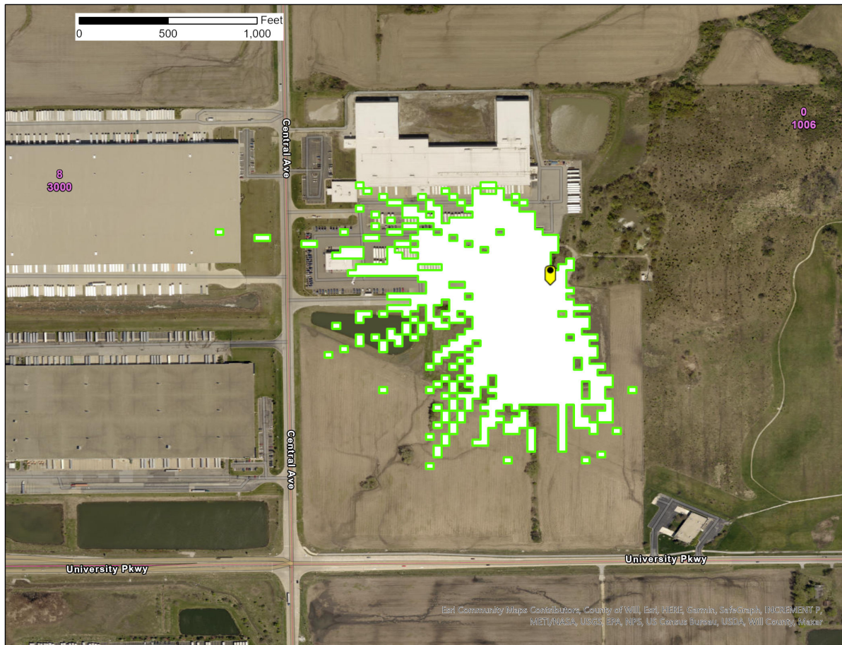
Figure 1 – Monee, IL SAN -77.6 \text{ dB(mW/(m}^2 * \text{ MHz))} pfd contour
