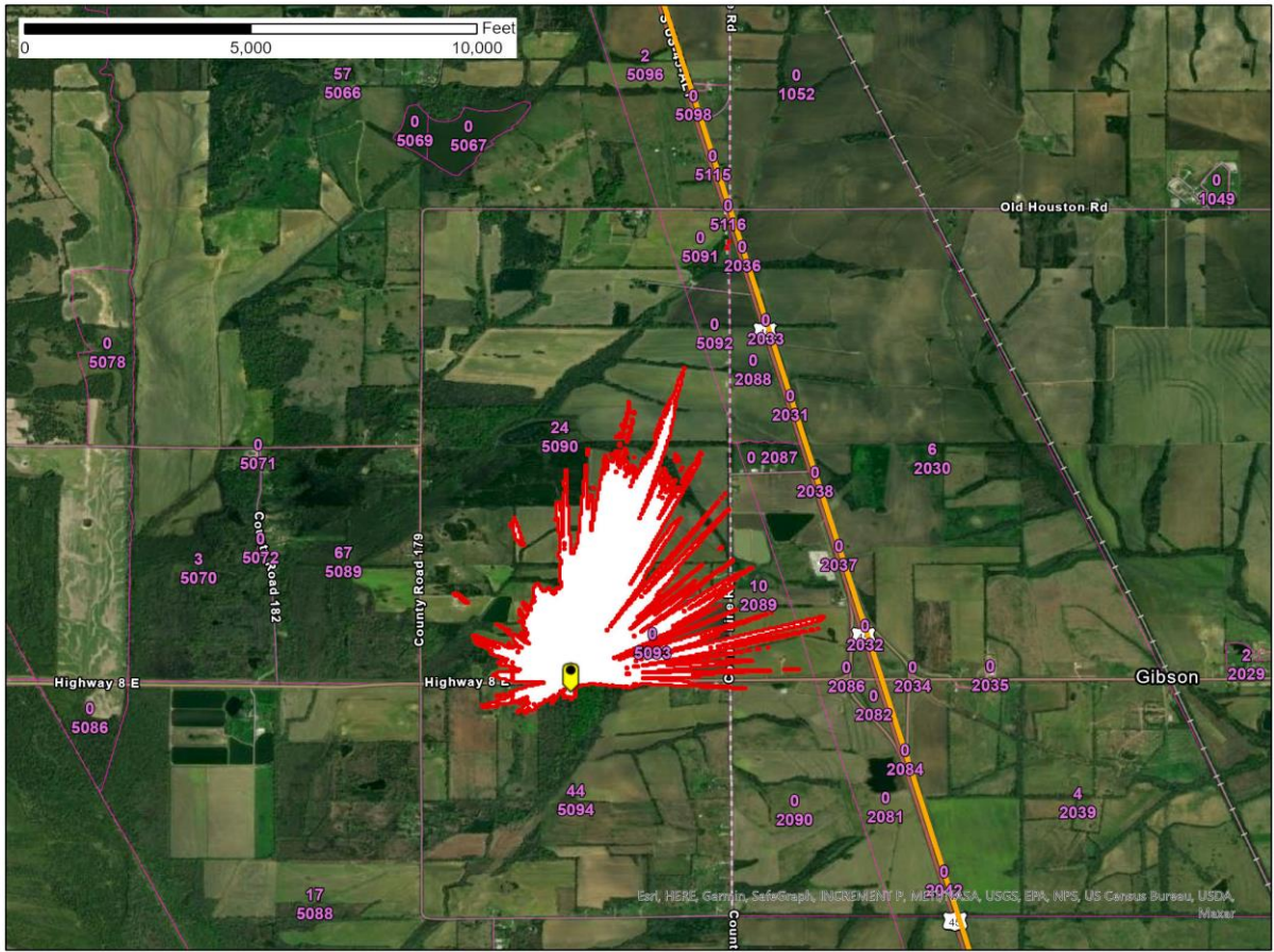
Figure 1 – Okolona, MS SAN -77.6 dB(mW/(m2 * MHz)) pfd contour
