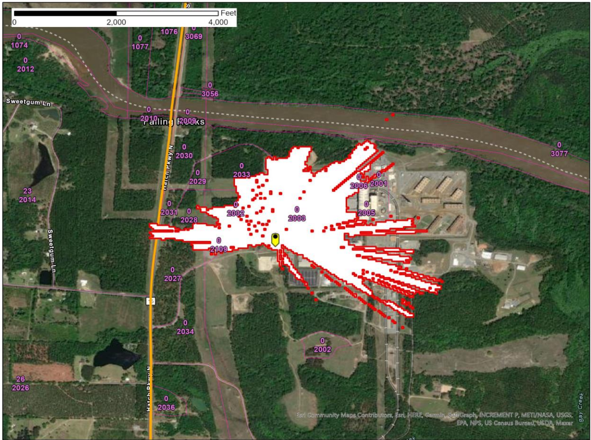
Figure 1 – Tarrytown, GA SAN -77.6 dB(mW/(m2 * MHz)) pfd contour
