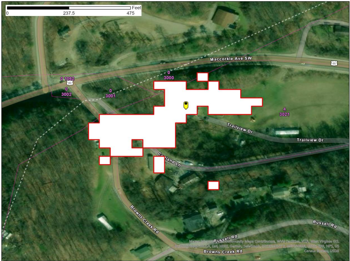
Figure 1 – St Albans, WV SAN -77.6 dB(mW/(m2 * MHz)) pfd contour
