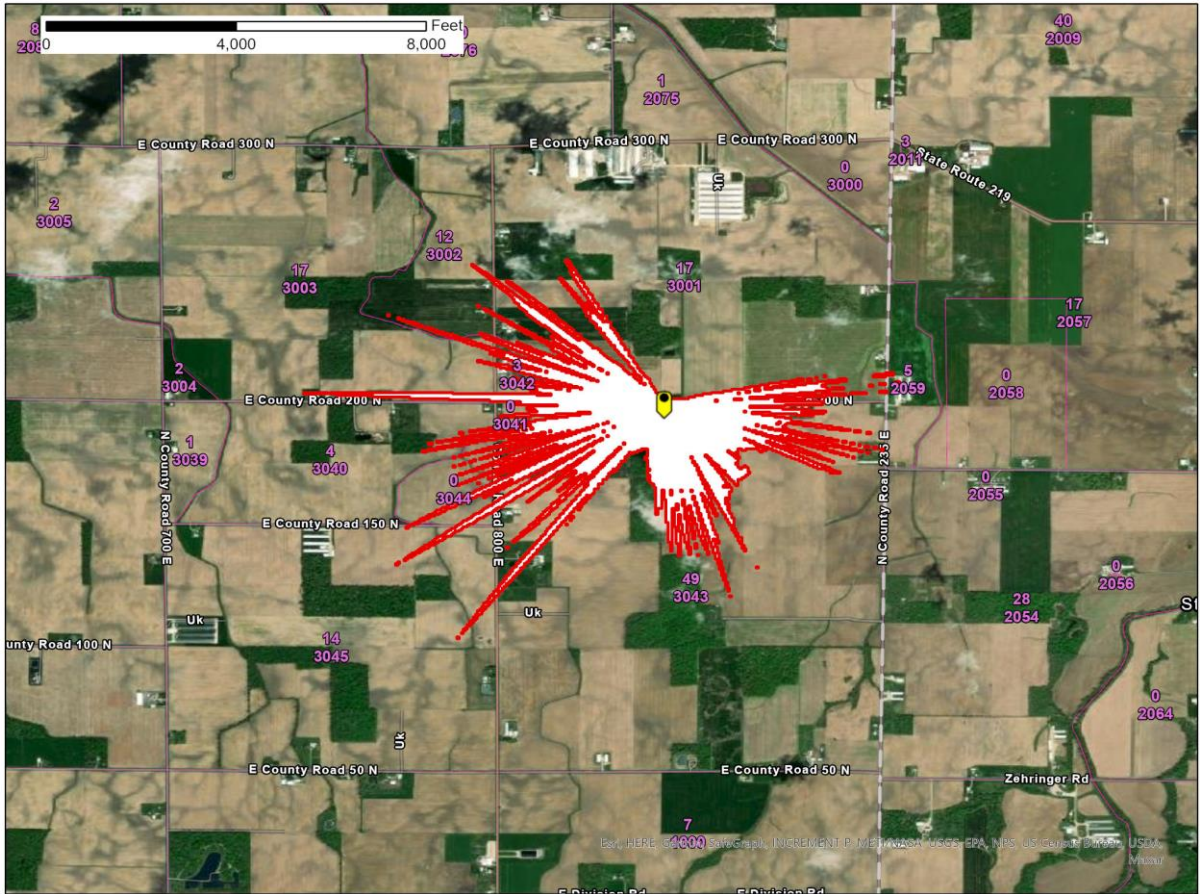
Figure 1 – PORTLAND, IN SAN -77.6 dB(mW/(m2 * MHz)) pfd contour
