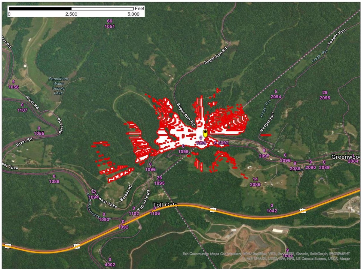
Figure 1 – Pennsboro, WV SAN -77.6 dB(mW/(m2 * MHz)) pfd contour
