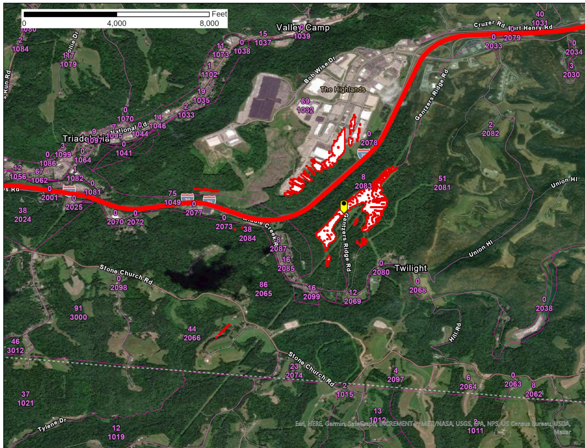
Figure 1 – Triadelphia, WV SAN -77.6 \text{ dB(mW/(m}^2 * \text{MHz))} pfd contour
