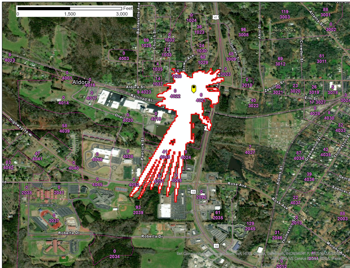
Figure 1 – Barnesville, GA SAN -77.6 \text{ dB(mW/(m}^2 * \text{ MHz))} pfd contour
