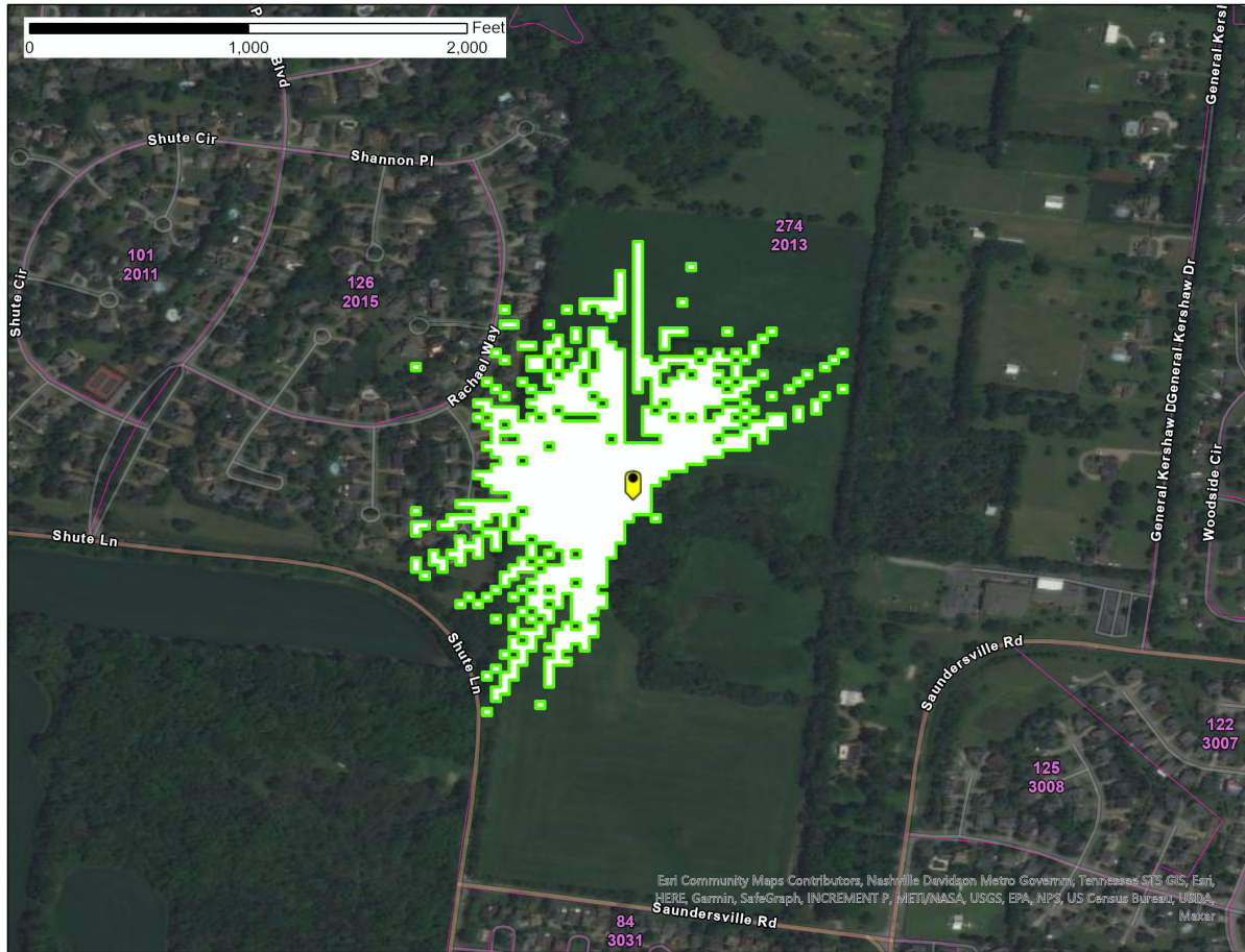
Figure 1 – Nashville, TN SAN -77.6 dB(mW/(m 2 * MHz)) pfd contour
