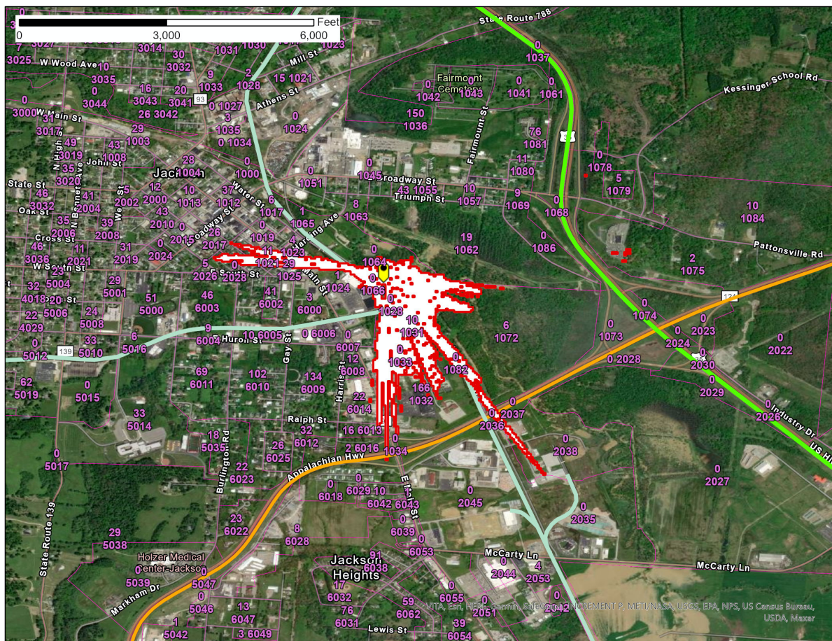
Figure 1 – Jackson, OH SAN -77.6 \text{ dB(mW/(m}^2 * \text{ MHz))} pfd contour
