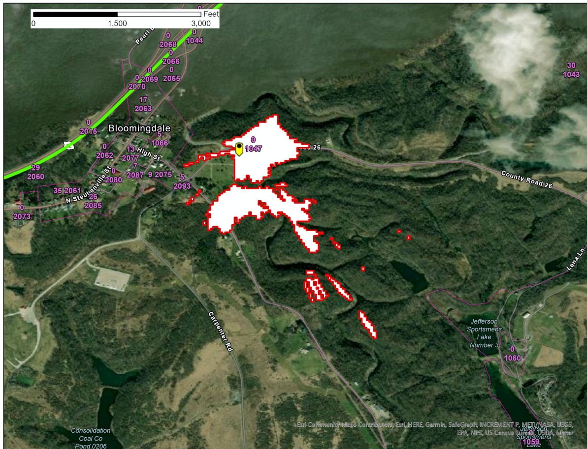
Figure 1 – Bloomingdale, OH SAN -77.6 \text{ dB(mW/(m}^2 * \text{MHz))} pfd contour
