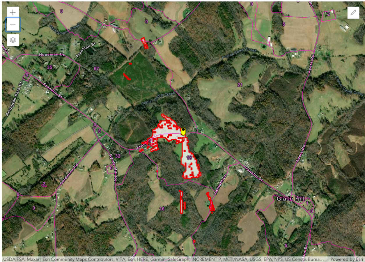
Figure 1 – Glade Hill, VA SAN -77.6 dB(mW/(m 2 * MHz)) pfd contour
