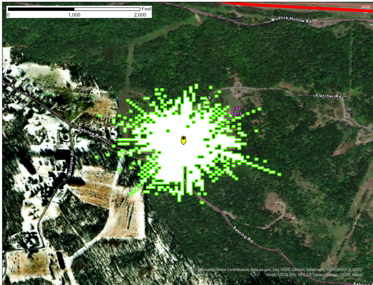
Figure 1 – Beaver, PA SAN -77.6 \text{ dB(mW/(m}^2 * \text{MHz))} pfd contour
