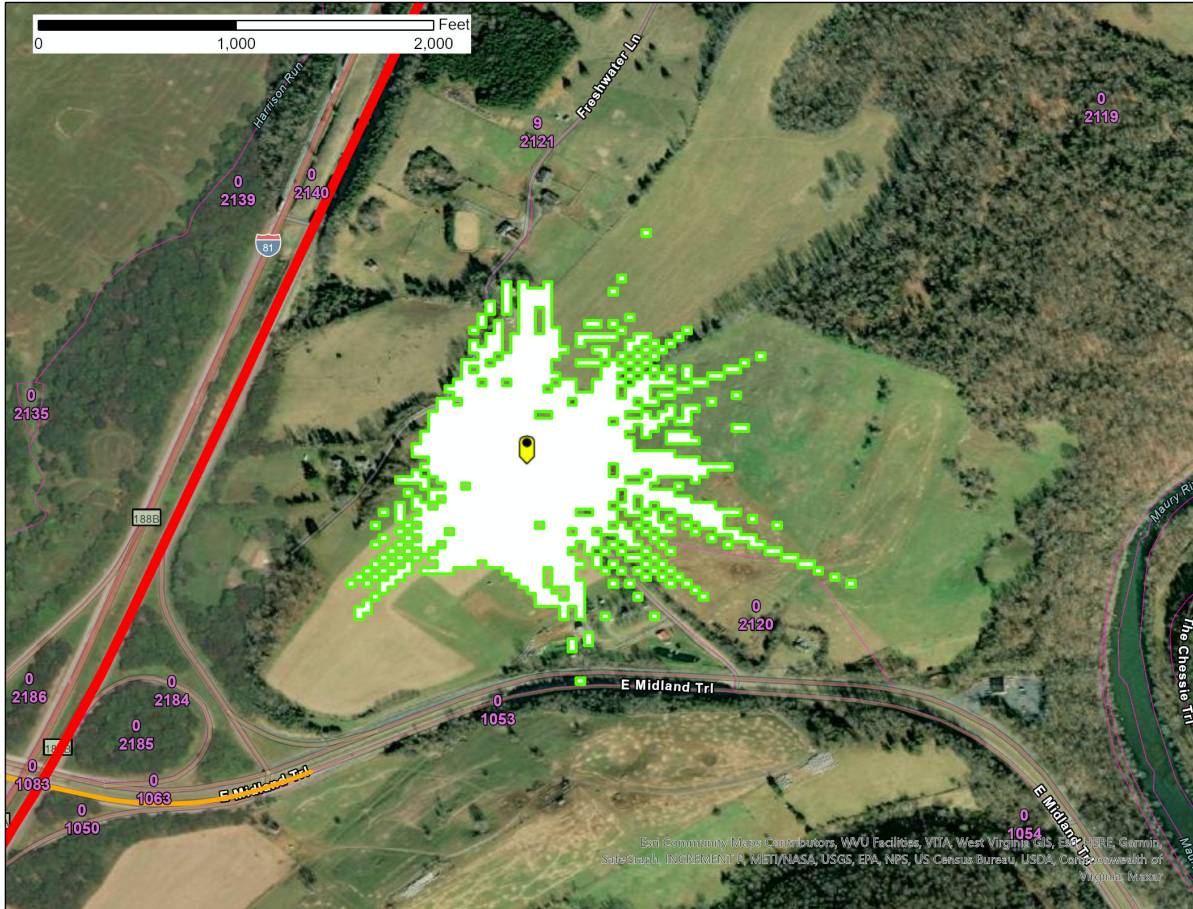
Figure 1 – Lexington, VA SAN -77.6 \text{ dB(mW/(m}^2 * \text{MHz))} pfd contour
