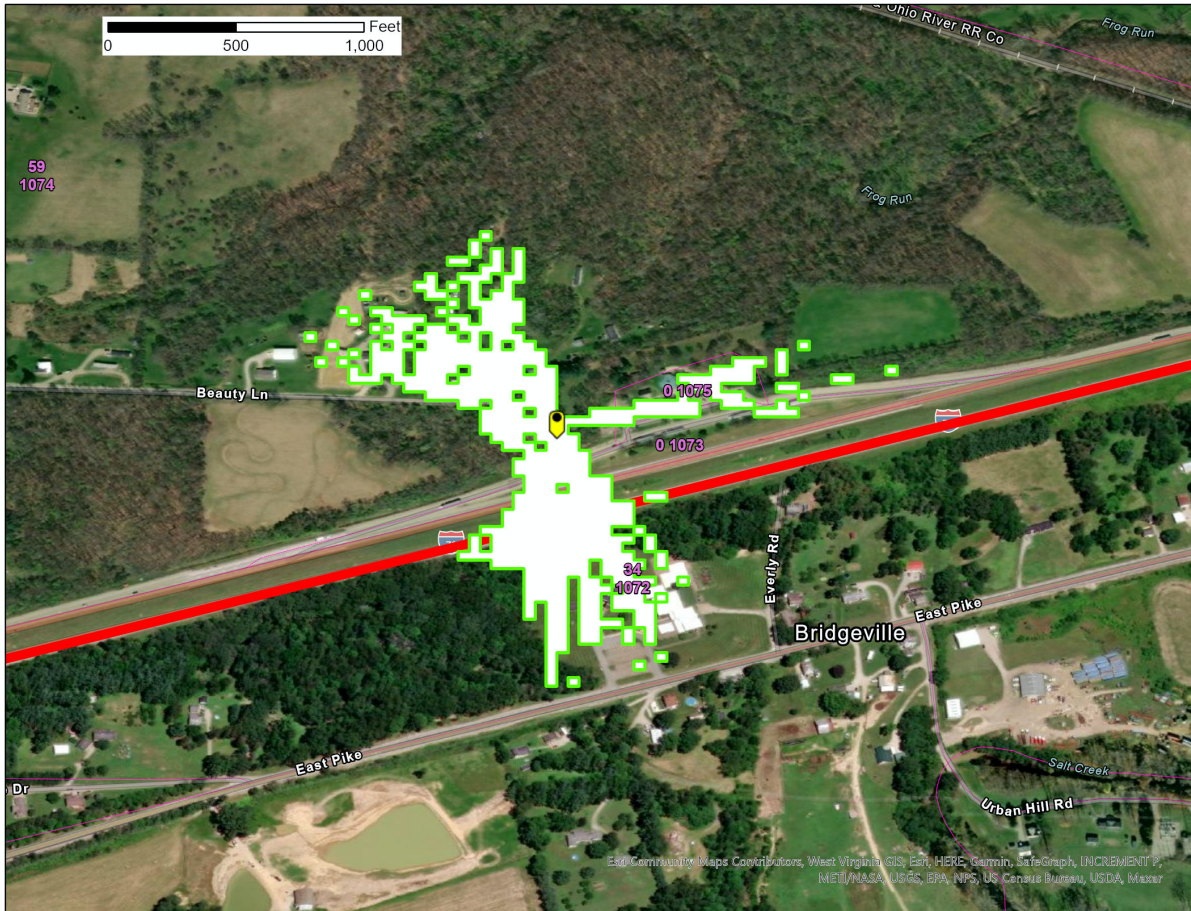
Figure 1 – Zanesville, OH SAN -77.6 \text{ dB(mW/(m}^2 * \text{MHz))} pfd contour
