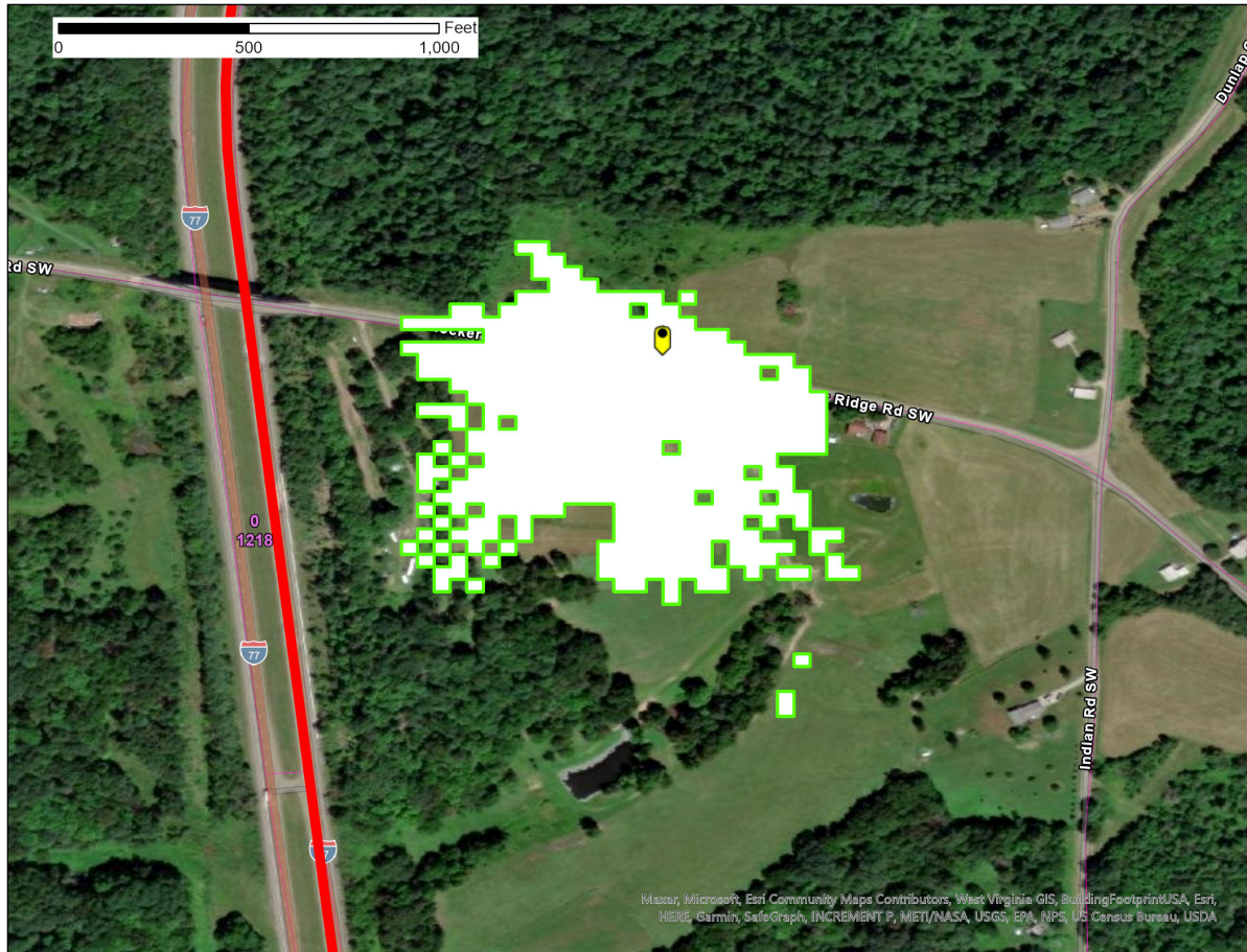
Figure 1 – Newcomerstown, OH SAN -77.6 \text{ dB(mW/(m}^2 * \text{MHz))} pfd contour
