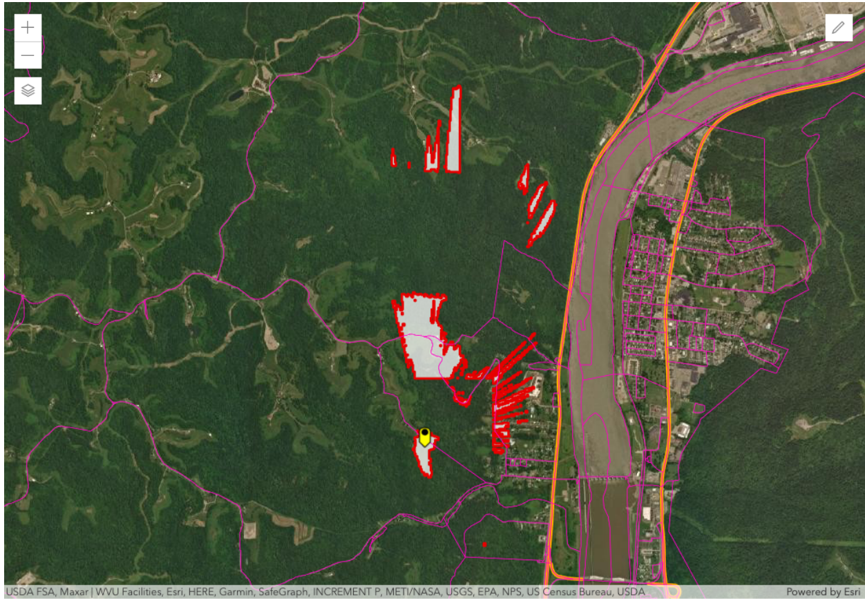
Figure 1 – Clarington, OH SAN -77.6 dB(mW/(m 2 * MHz)) pfd contour
