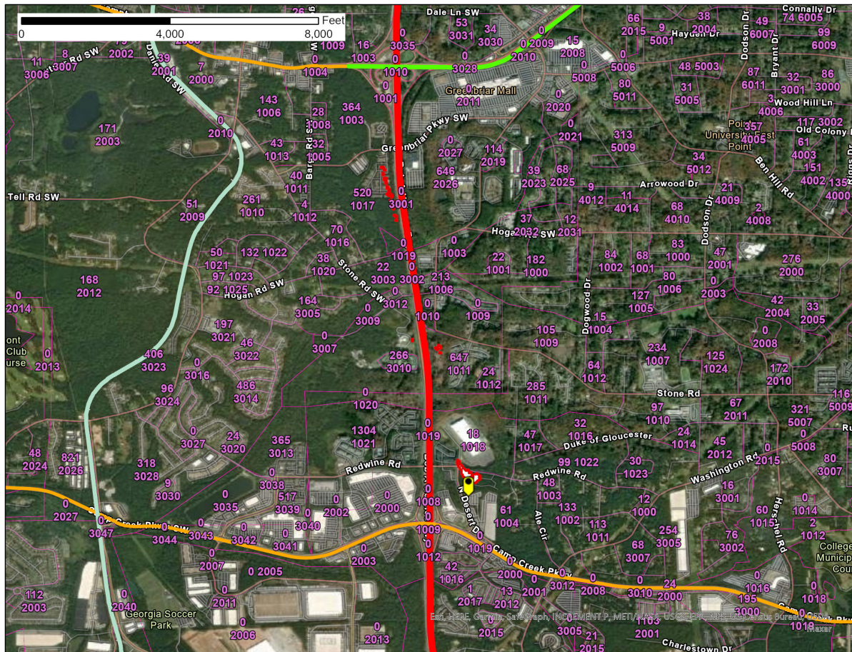
Figure 1 – East Point, GA SAN -77.6 \text{ dB(mW/(m}^2 * \text{MHz))} pfd contour
