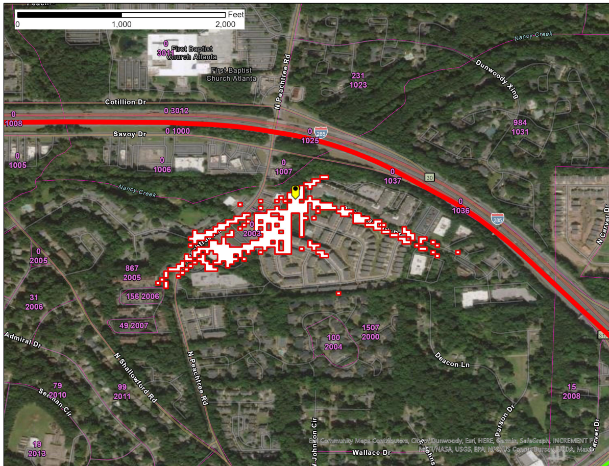
Figure 1 – Chamblee, GA SAN -77.6 \text{ dB(mW/(m}^2 * \text{MHz))} pfd contour
